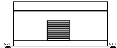
ELEVATION PLAN
