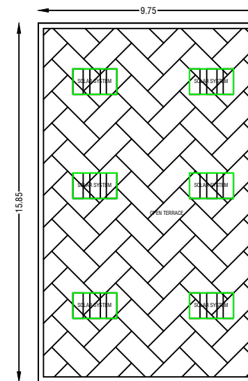
OPEN TERRACE PLAN
