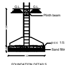
FOUNDATION DETAILS
