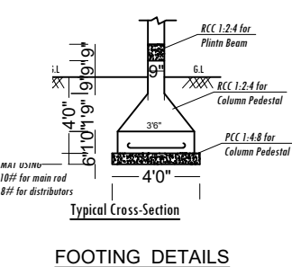
FOOTING DETAILS
