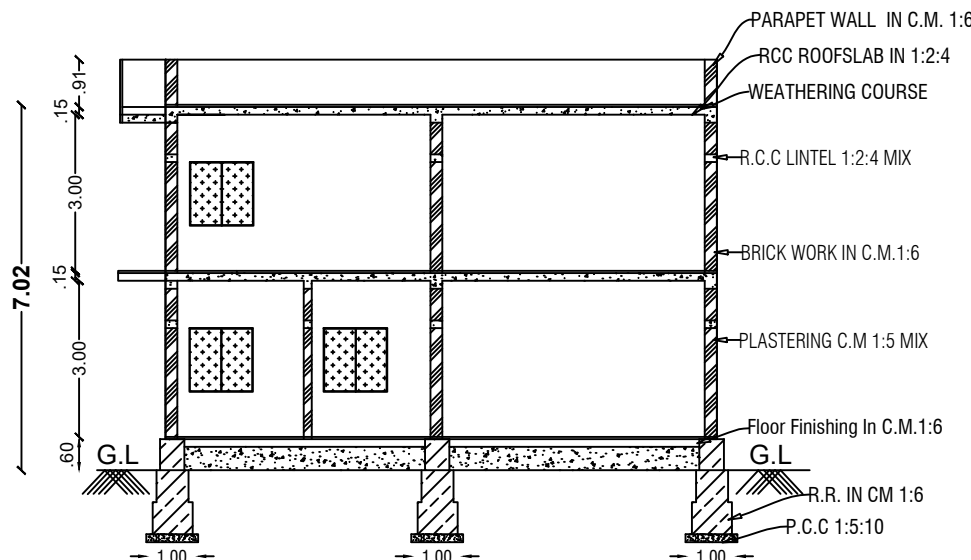
SECTION ON-\"AB\"
