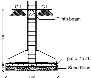
FOUNDATION DETAILS
