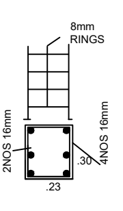
COLUMN DETAILS (NOT TO SCALE)
