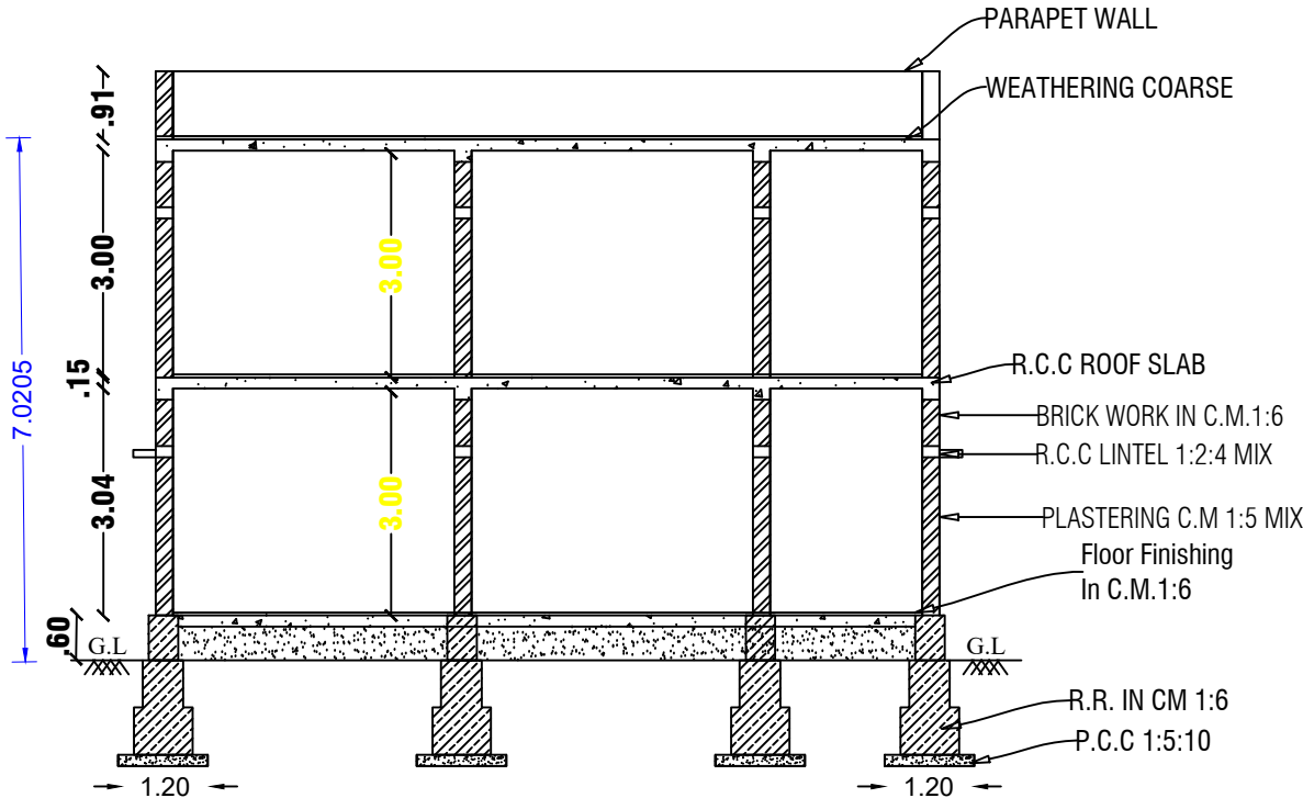
SECTION ON-'AB'
