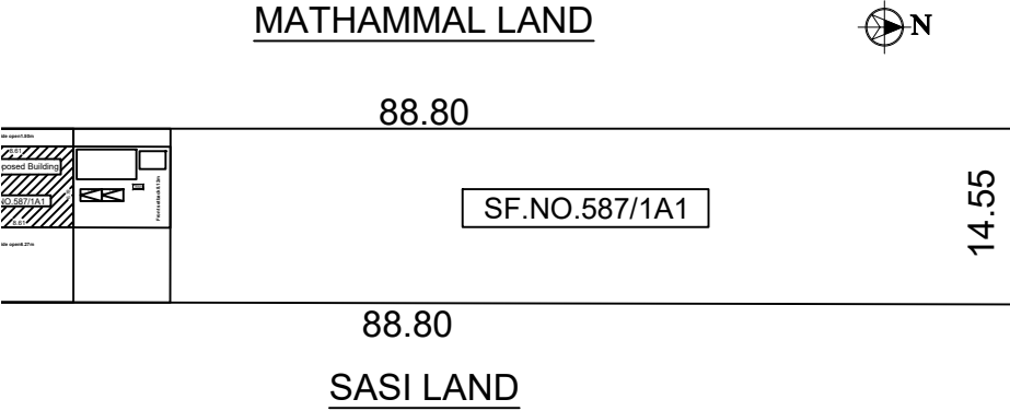
SITE PLAN SCALE 1:100 & As Per FMB
