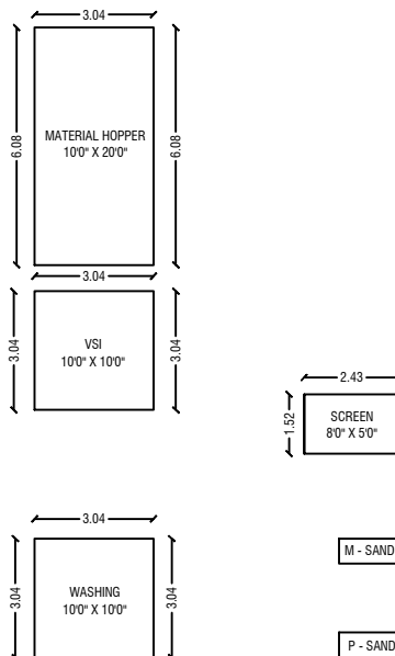
PLAN
