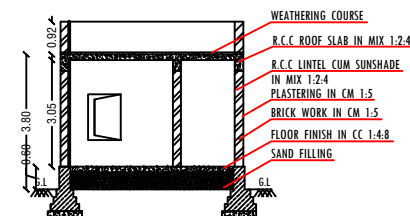
SECTION ON-AA'
