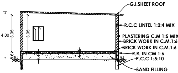
Section On-"AB"
