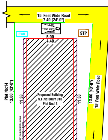
SITE PLAN Scale: 1:100 As Per Document
