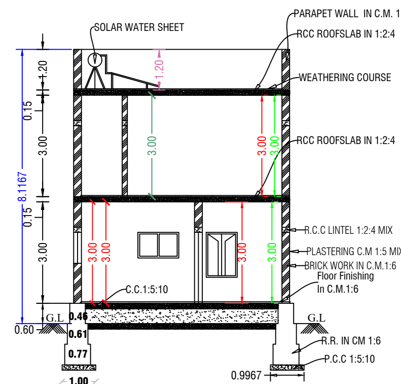
Section On-'AA'
