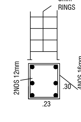
COLUMN DETAILS (NOT TO SCALE)
