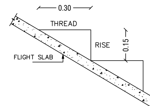
STAIRCASE DETAILS
