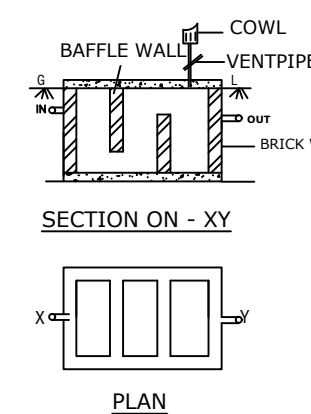
SEPTICTANK DETAILS NOT TO SCALE
