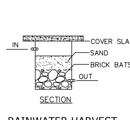
RAINWATER HARVEST NOT TO SCALE
