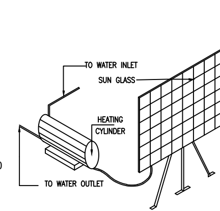
SOLAR WATER HEATING SYSTEM SCALE: 1:N.T.S.
