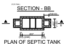
PLAN OF SEPTIC TANK
