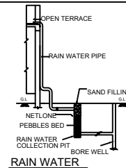
RAIN WATER
