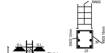
COLUMN DETAILS
