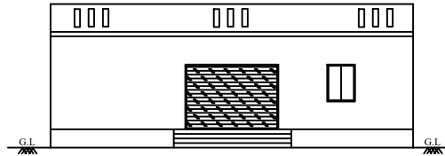
FRONT ELEVATION
