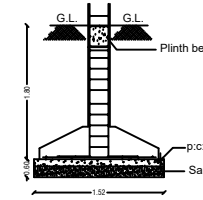
FOUNDATION DETAILS
