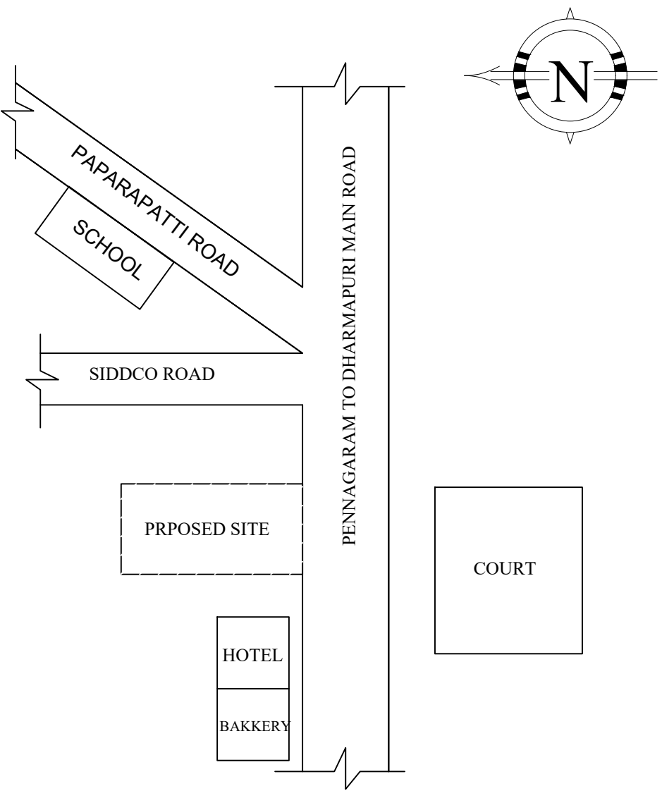
LOCATION PLAN
