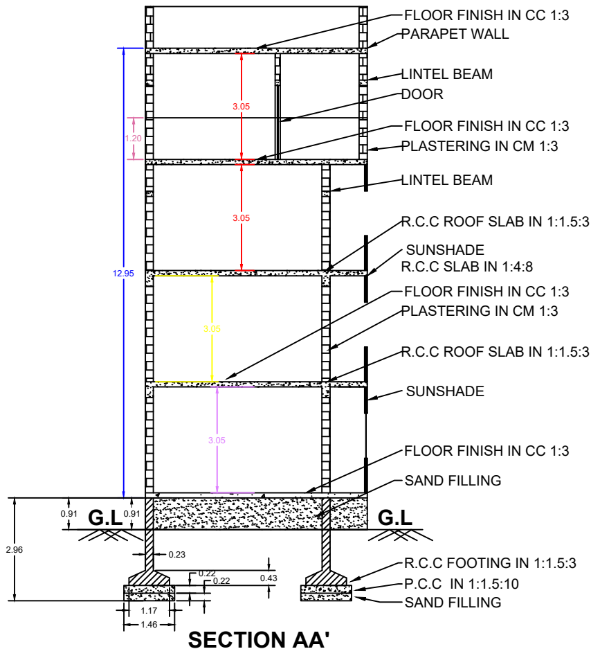
SECTION AA'
