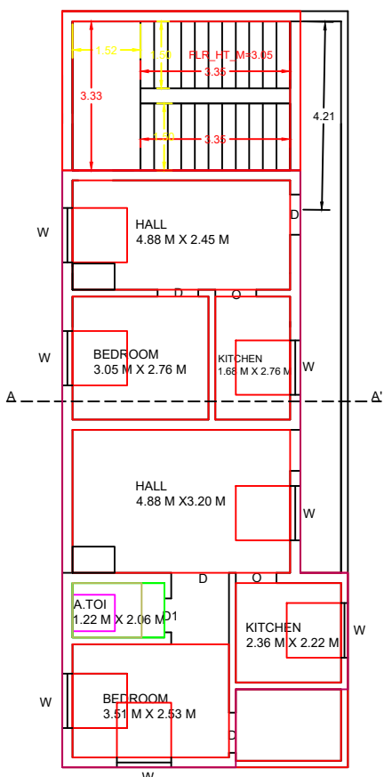
SECOND FLOOR
