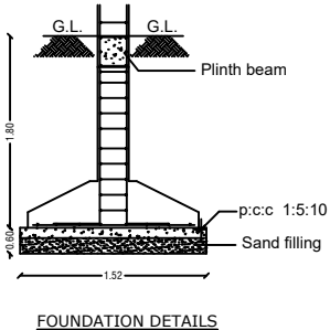
FOUNDATION DETAILS
