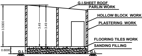
SECTION "AB"
