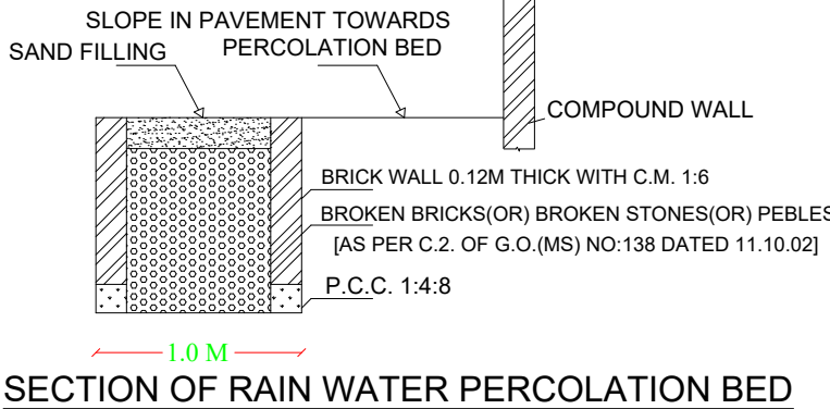
SECTION OF RAIN WATER PERCOLATION BED
