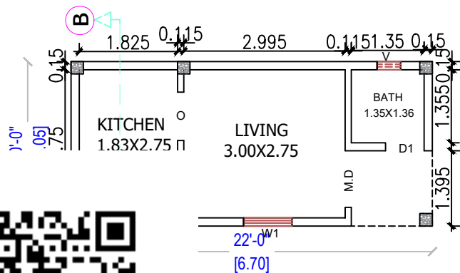
IND FLOOR PLAN (Scale 1:100)
