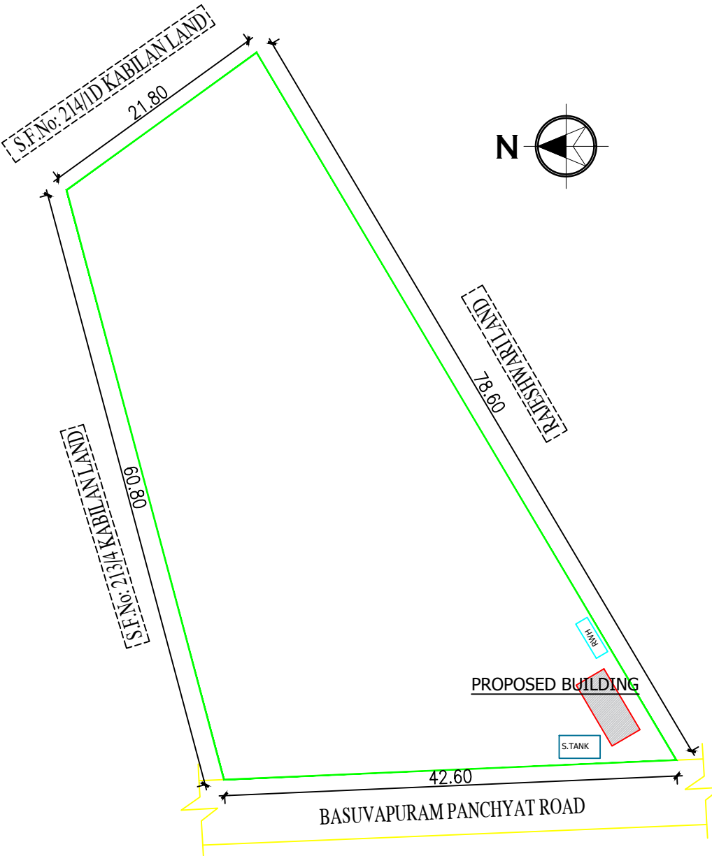
SITE PLAN FOR PROPOSED BUILDING (Scale 1:500)
