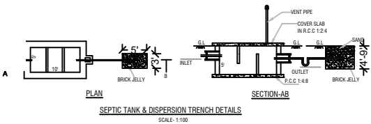
SEPTIC TANK & DISPERSION TRENCH DETAILS SCALE- 1:50
