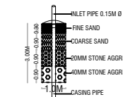
DETAILS OF RAIN WATER HARVESTING STRUCTURES
