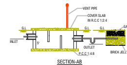
SECTION-AB
