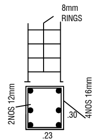
COLUMN DETAILS (NOT TO SCALE)
