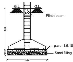
FOUNDATION DETAILS
