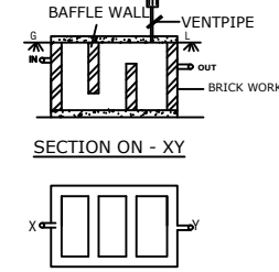
SEPTICTANK DETAILS NOT TO SCALE
