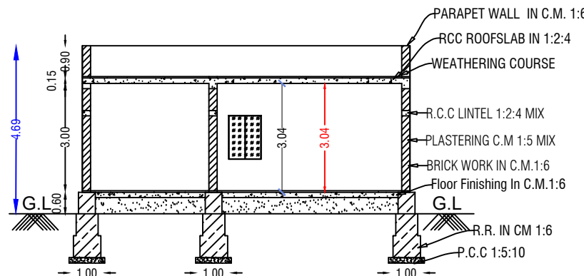
SECTION ON-'AB'
