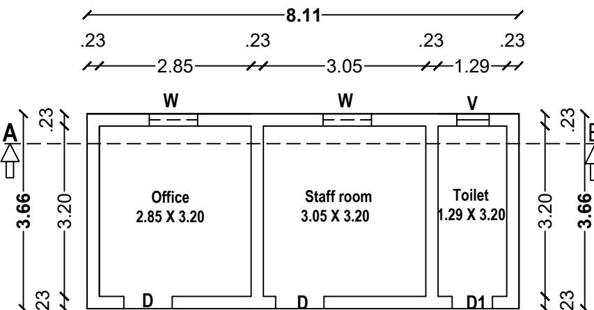
Block-II Ground Floor Plan
