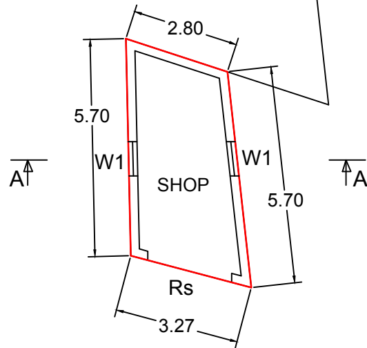
PLAN
