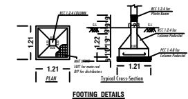
FOOTING DETAILS
