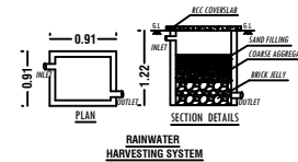
RAINWATER HARVESTING SYSTEM
