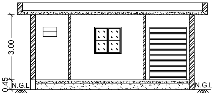
SECTION ON-"AB"
