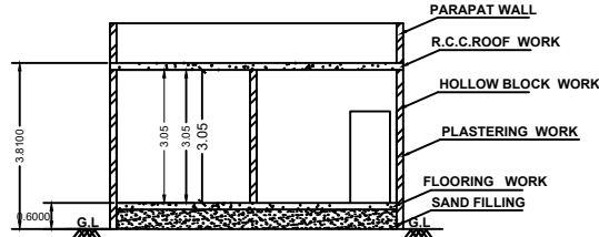
SECTION "AB"
