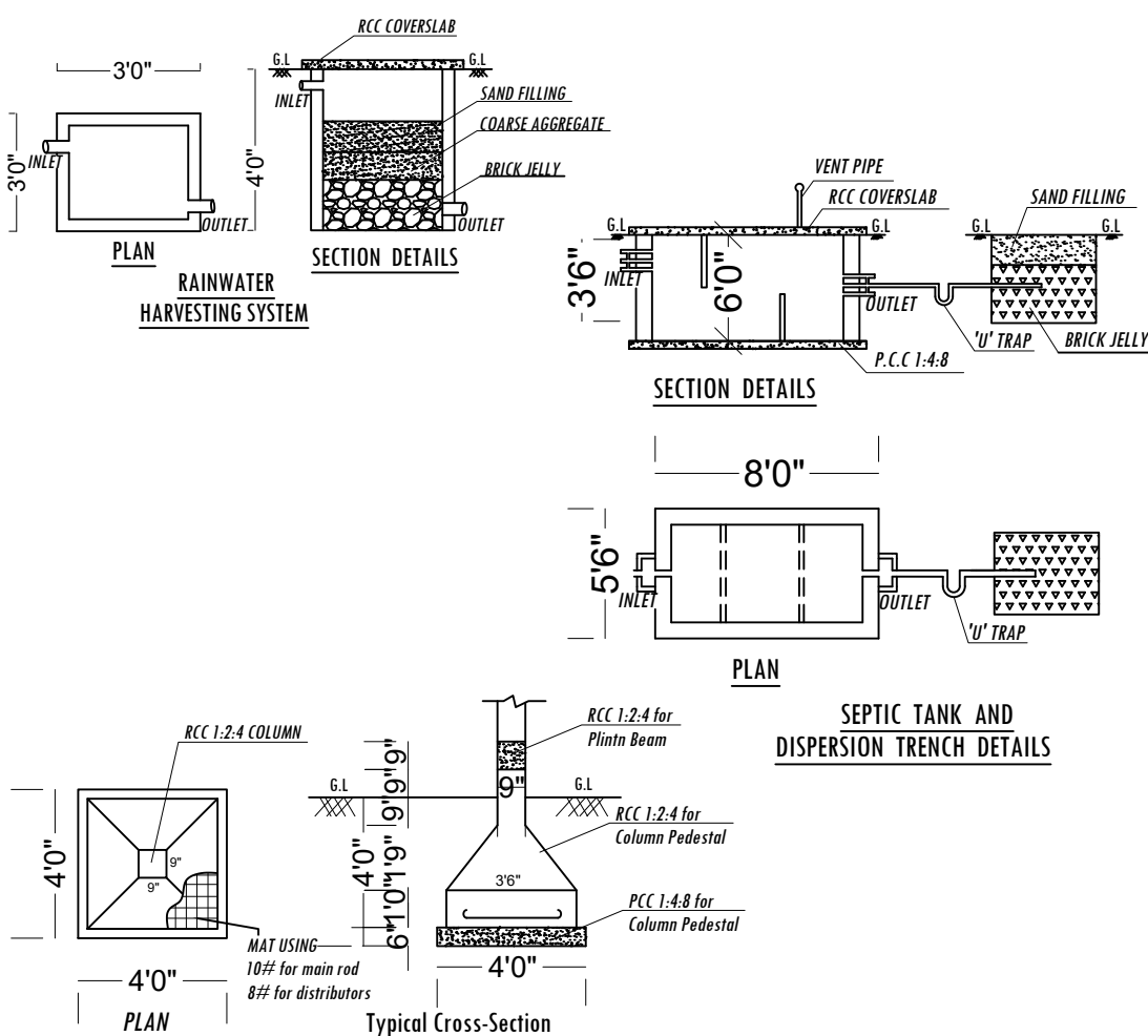
FOOTING DETAILS
