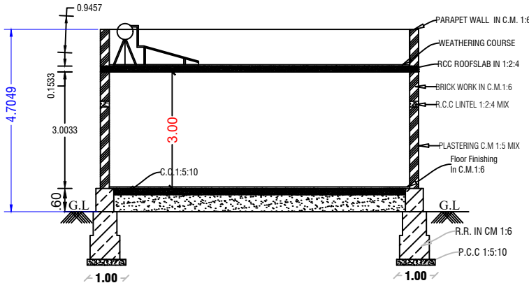
SECTION ON-AB
