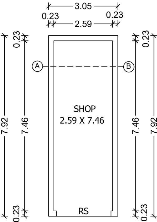
GROUND FLOOR PLAN EAST FACEING
