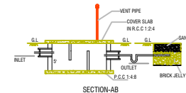
SEPTIC TANK & DISPERSION TRENCH DETAILS SCALE- 1:100
