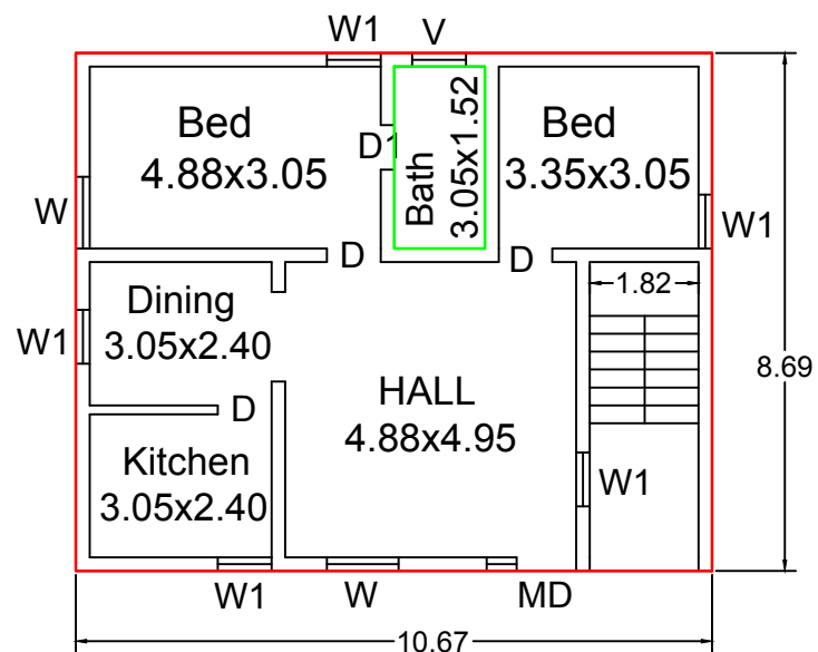
PLAN - Ground Floor
