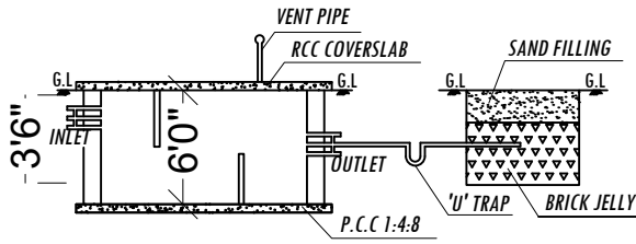
SEPTIC TANK AND DISPERSION TRENCH DETAILS
