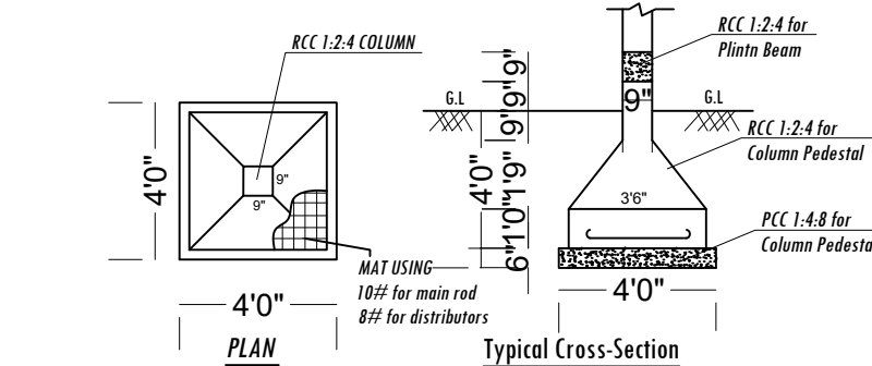
FOOTING DETAILS
