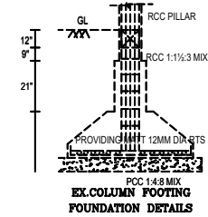
EX.COLUMN FOOTING
