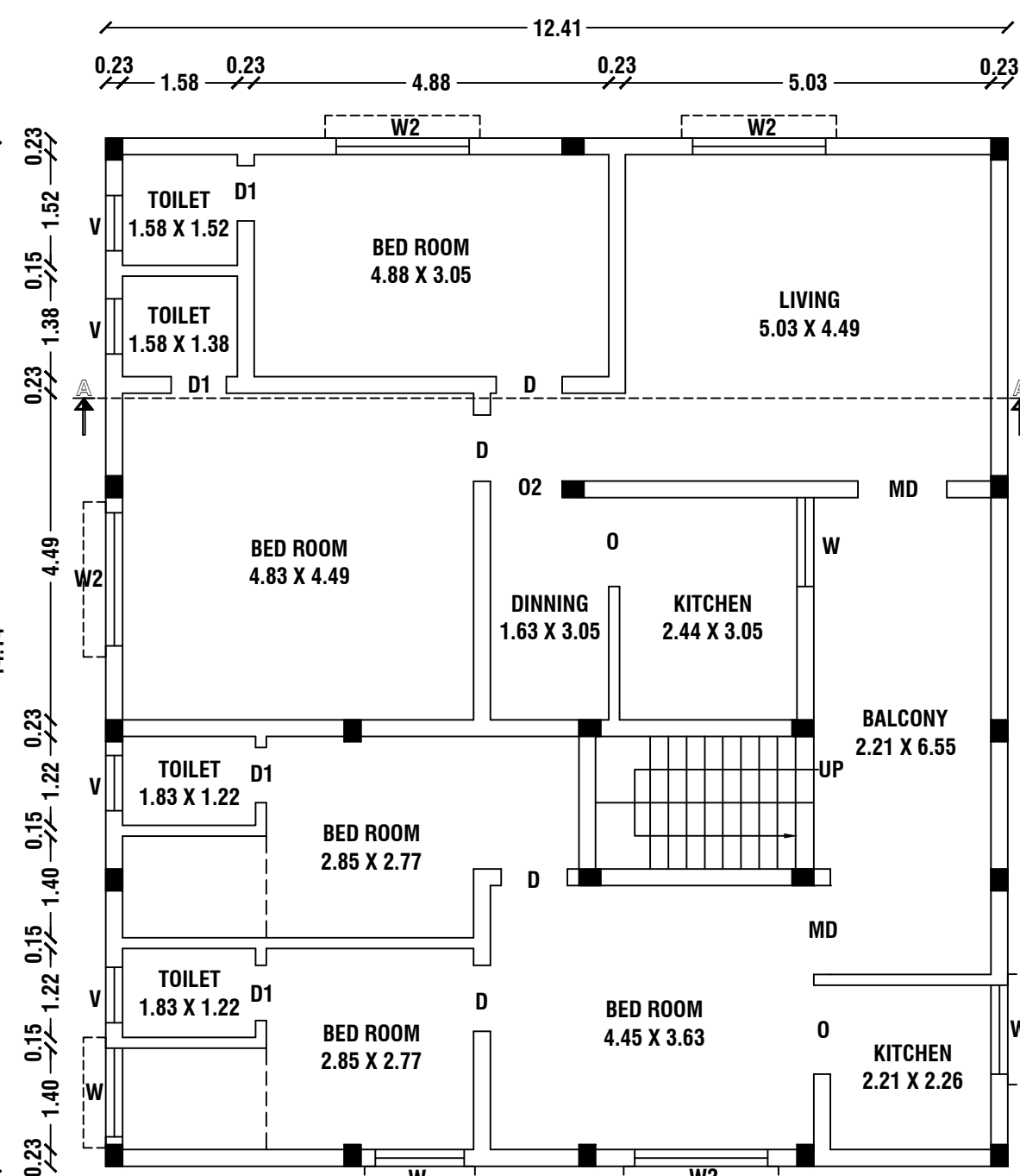
FIRST FLOOR PLAN (PROPOSED BUILDING)
