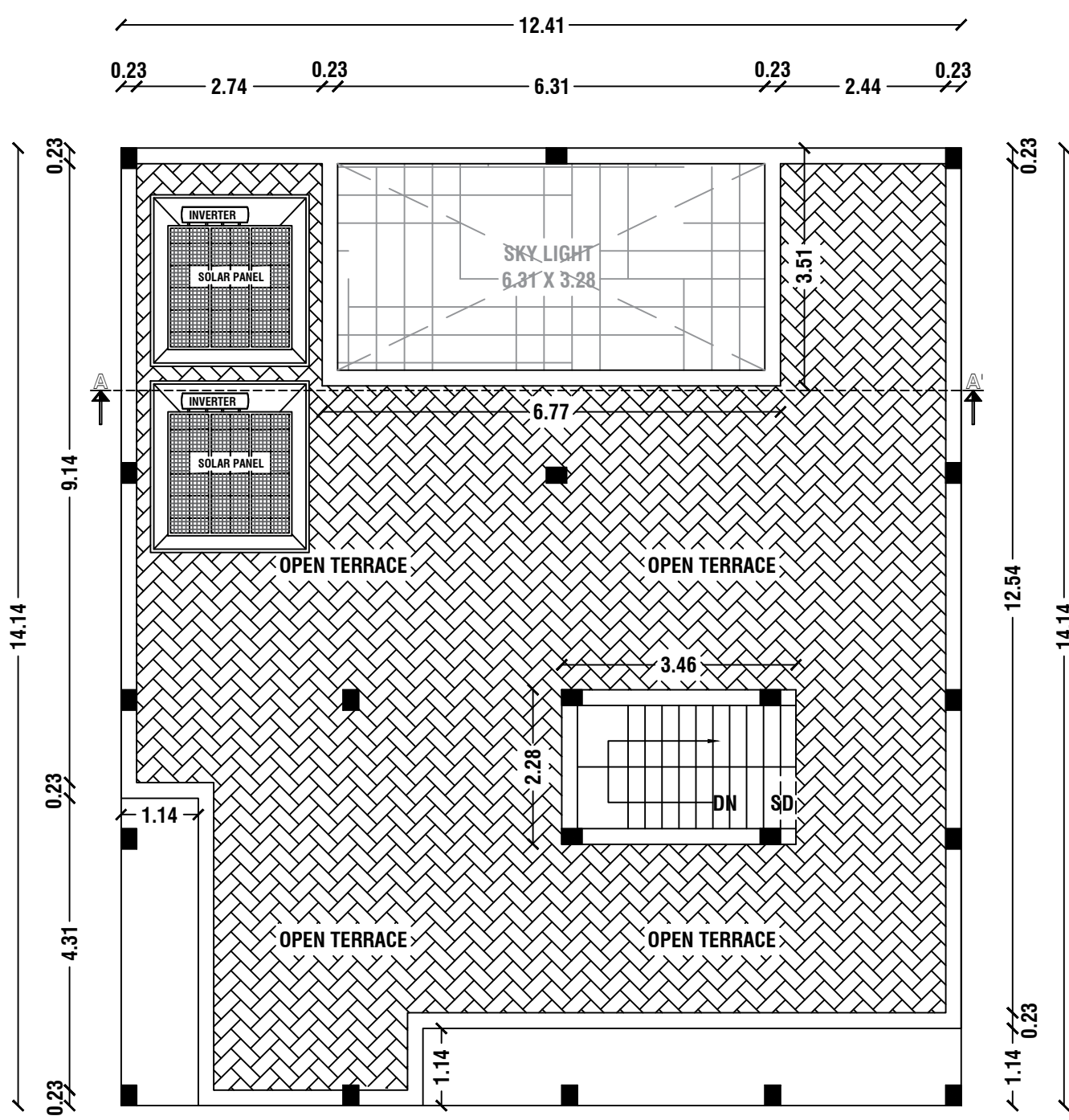
HEAD ROOM CUM OPEN TERRACE FLOOR PLAN (PROPOSED BUILDING)
