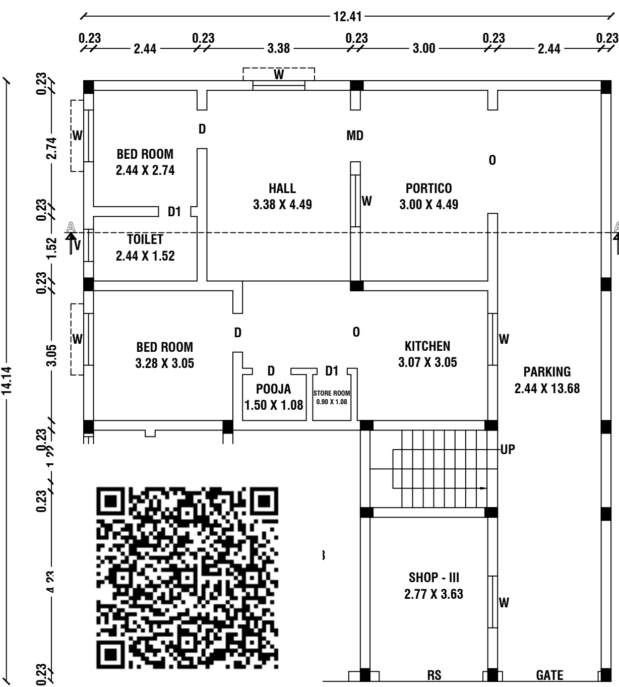
GROUND FLOOR PLAN (EXISTING BUILDING)
