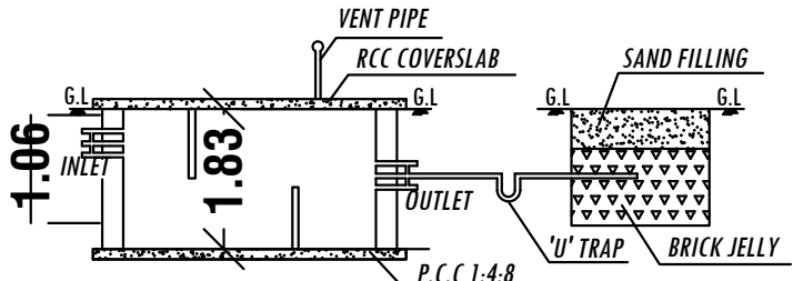
SECTION DETAILS
