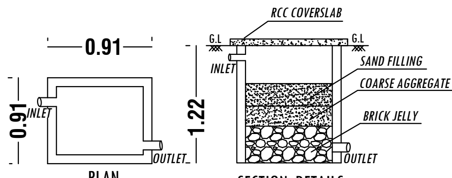
RAINWATER HARVESTING SYSTEM
