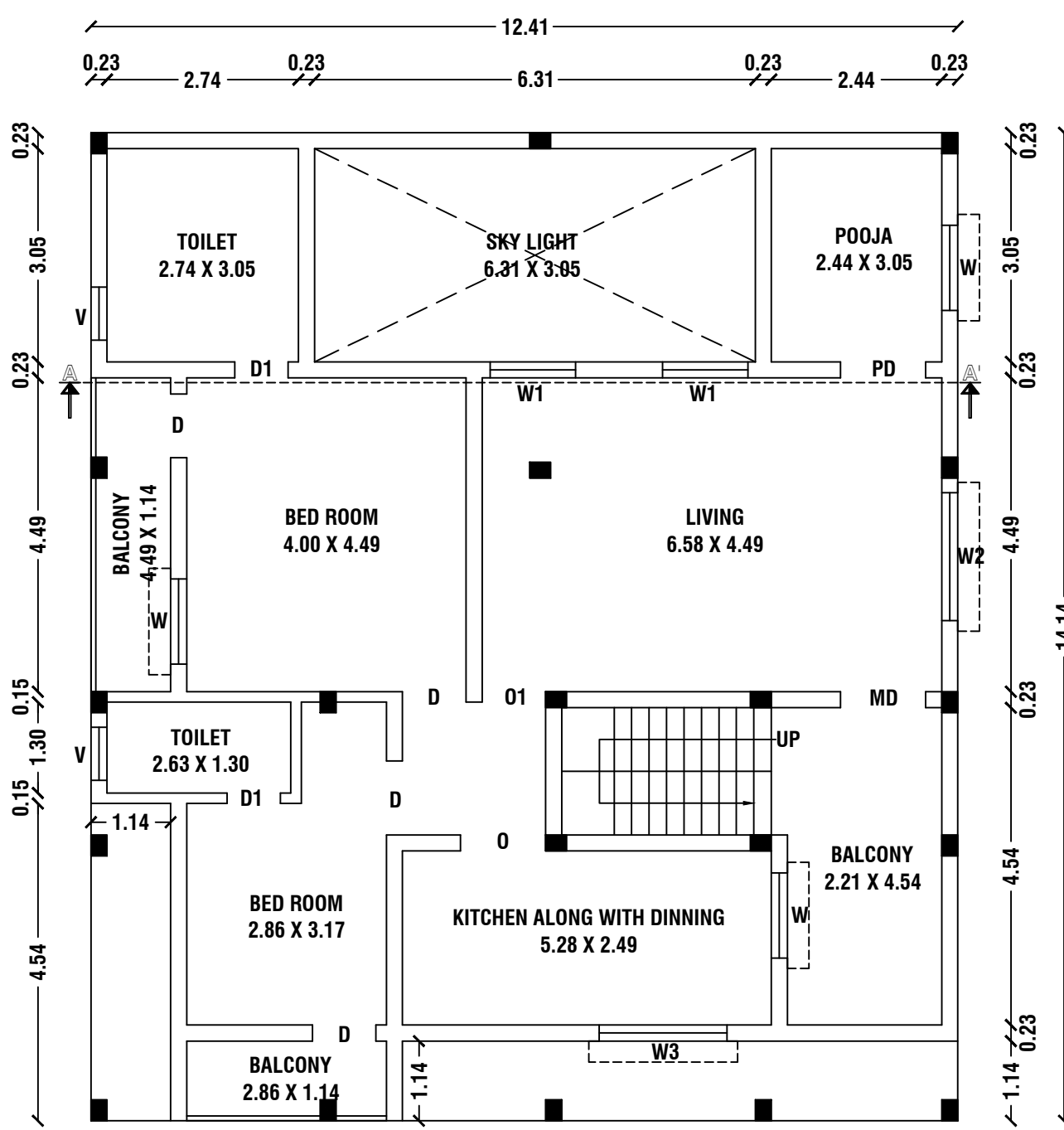
SECOND FLOOR PLAN (PROPOSED BUILDING)
