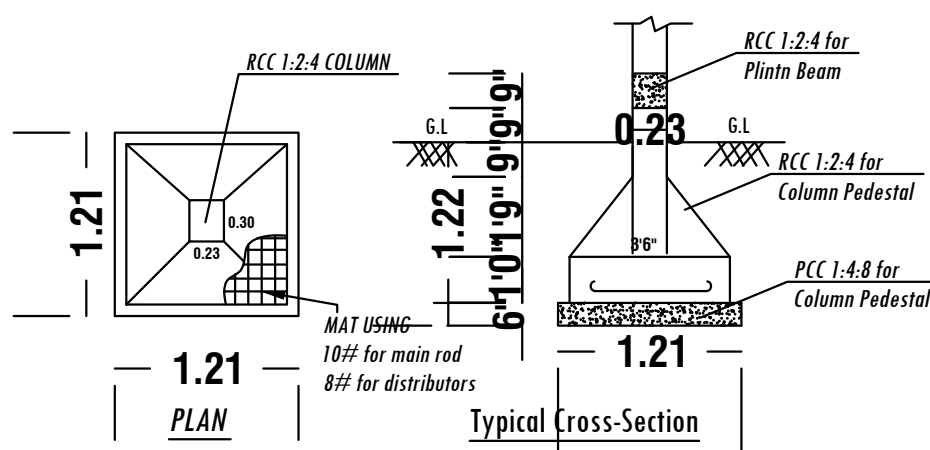
FOOTING DETAILS
