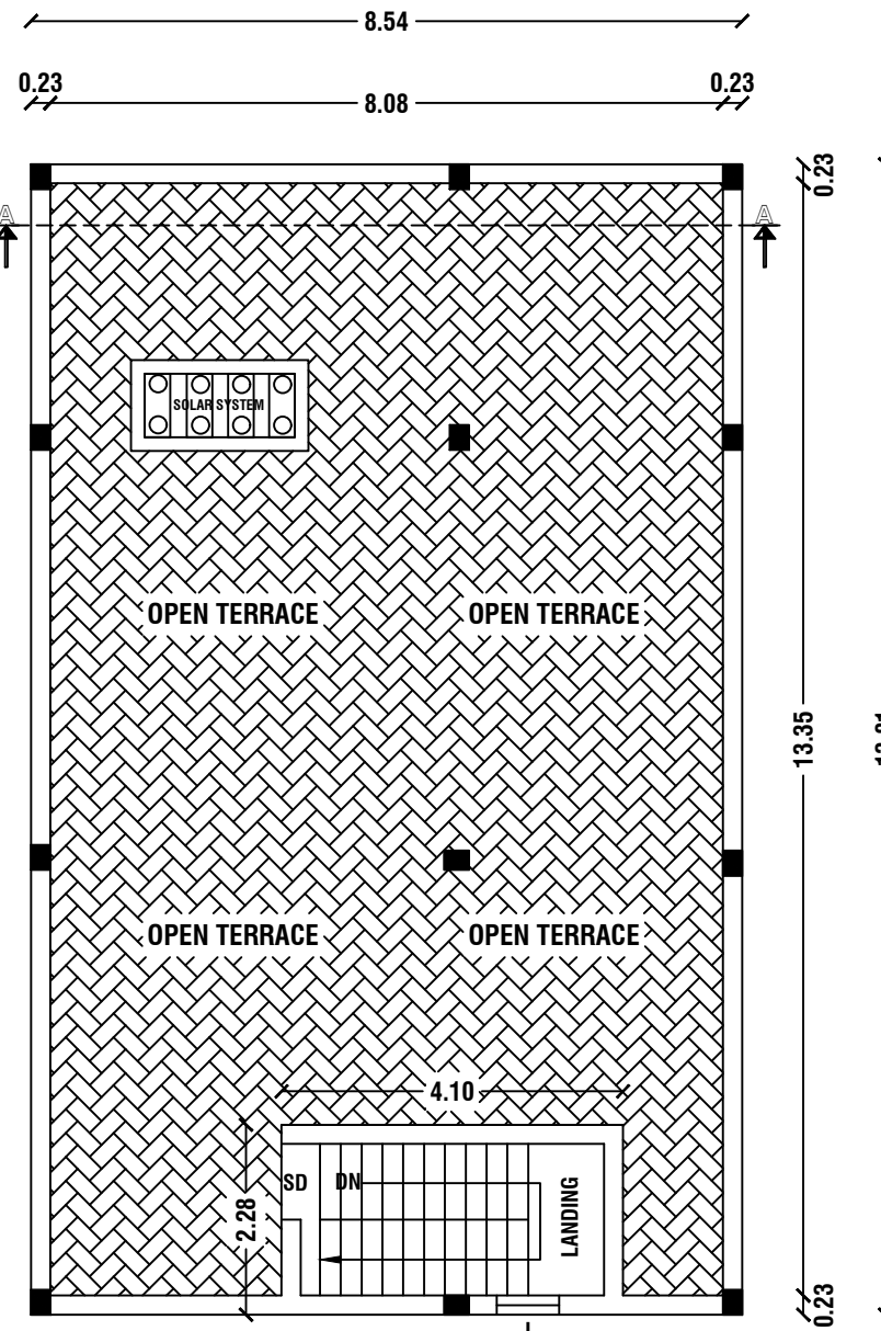
HEAD ROOM CUM OPEN TERRACE FLOOR PLAN
