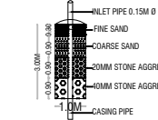
DETAILS OF RAIN WATER HARVESTING STRUCTURES
