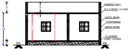
SECTION : "A-B"
