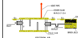
SECTION-AB
