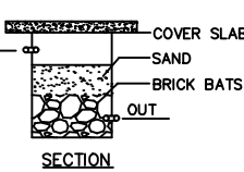
RAINWATER HARVEST
