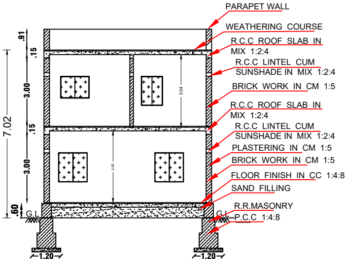
SECTION ON-"AB"
