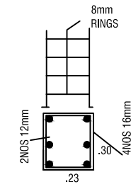
COLUMN DETAILS (NOT TO SCALE)
