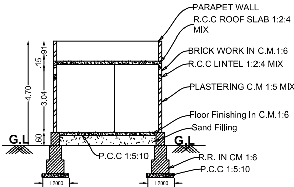
SECTION ON-"AB"
