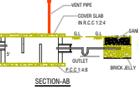
SECTION-AB
