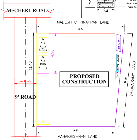
SITE PLAN
