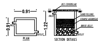
RAINWATER HARVESTING SYSTEM
