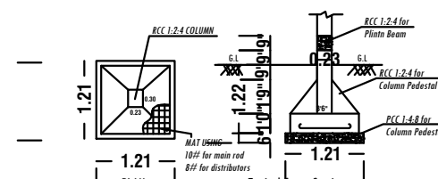
FOOTING DETAILS
