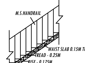
STAIR CASE DETAILS
