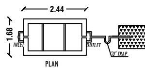
SEPTIC TANK AND DISPERSION TRENCH DETAILS
