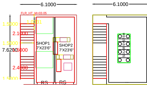
GROUND FLOOR PLAN SCALE 1:100 TERRACE FLOOR PLAN
