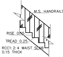
STAIRCASE DETAILS SCALE-1:20
