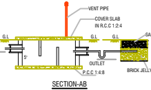
SECTION-AB
