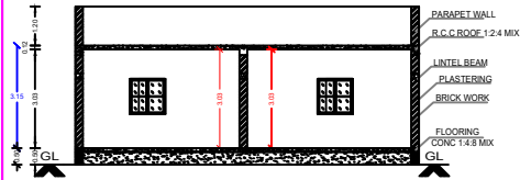
SECTION - "A-B"
