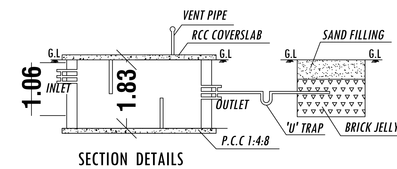
SECTION DETAILS
