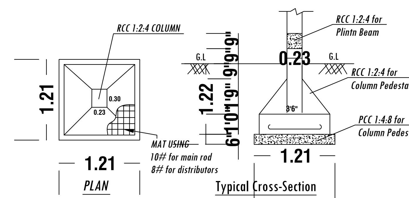
FOOTING DETAILS
