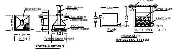
FOOTING DETAILS
