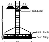
FOUNDATION DETAILS
