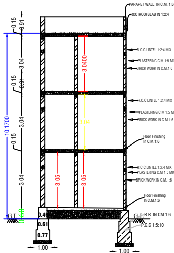
SECTION ON - 'AB'
