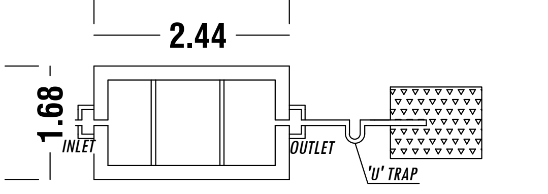
SEPTIC TANK AND DISPERSION TRENCH DETAILS
