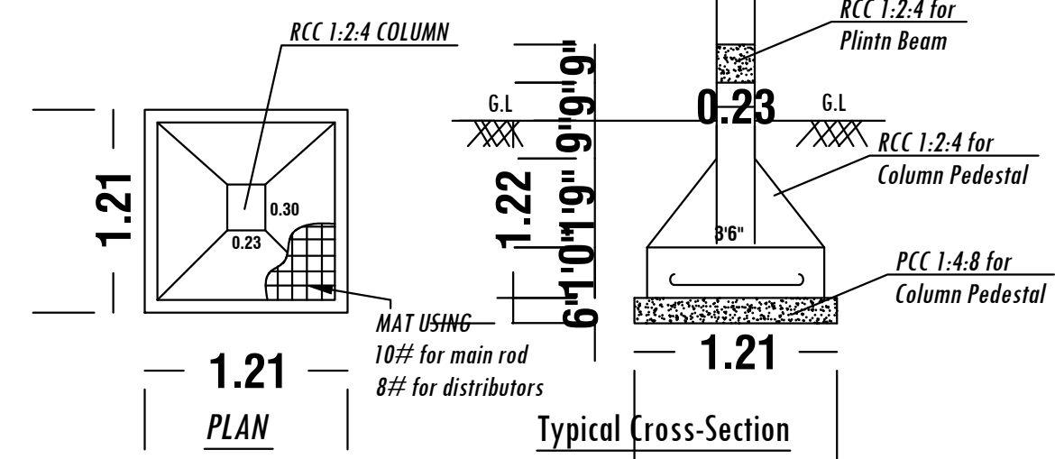
FOOTING DETAILS
