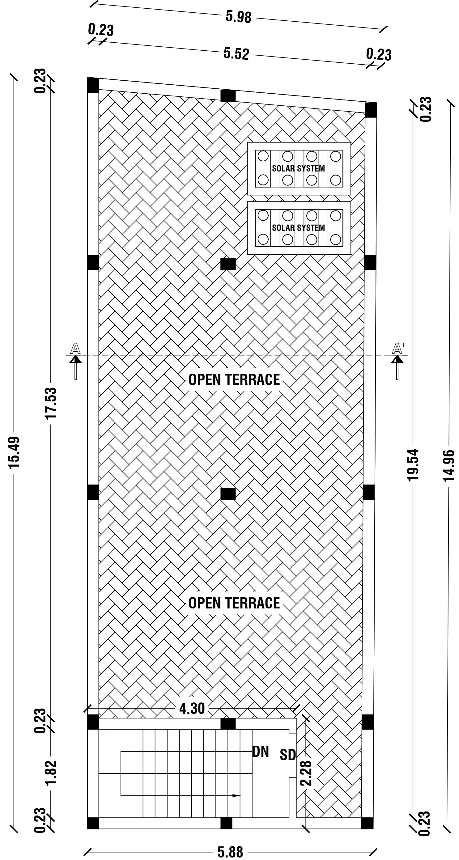
HEAD ROOM CUM OPEN TERRACE FLOOR PLAN
