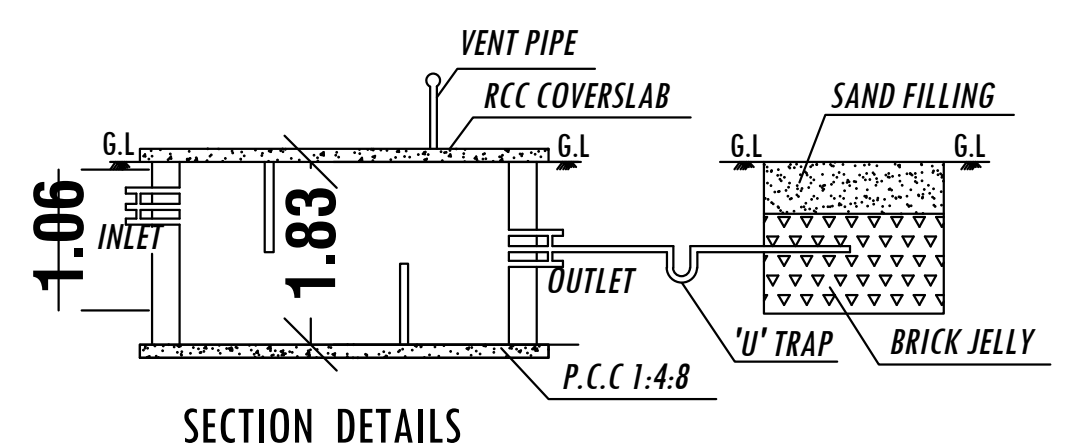
SECTION DETAILS
