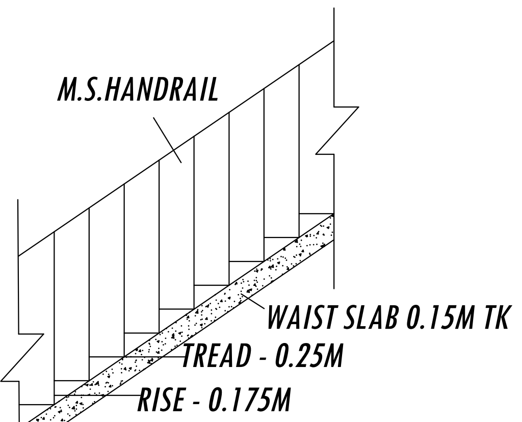
STAIR CASE DETAILS
