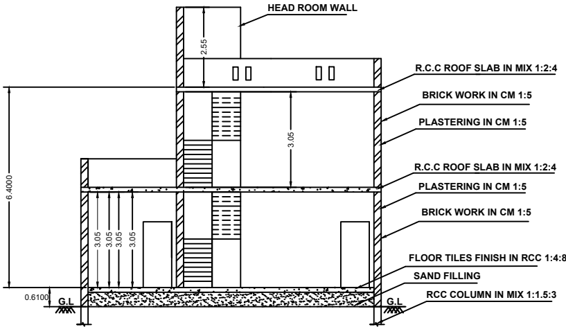
SECTION-AB
