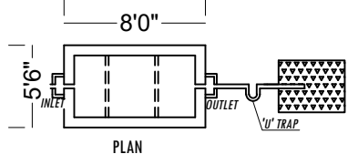
SEPTIC TANK AND DISPERSION TRENCH DETAILS
