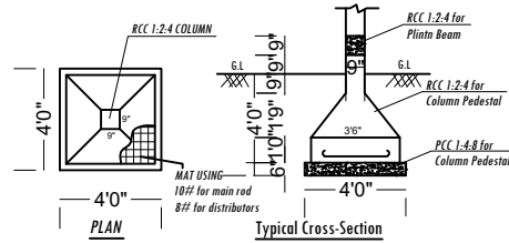
FOOTING DETAILS
