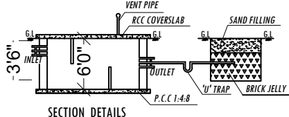
SECTION DETAILS
