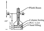
FOUNDATION DETAILS SCALE 1:50
