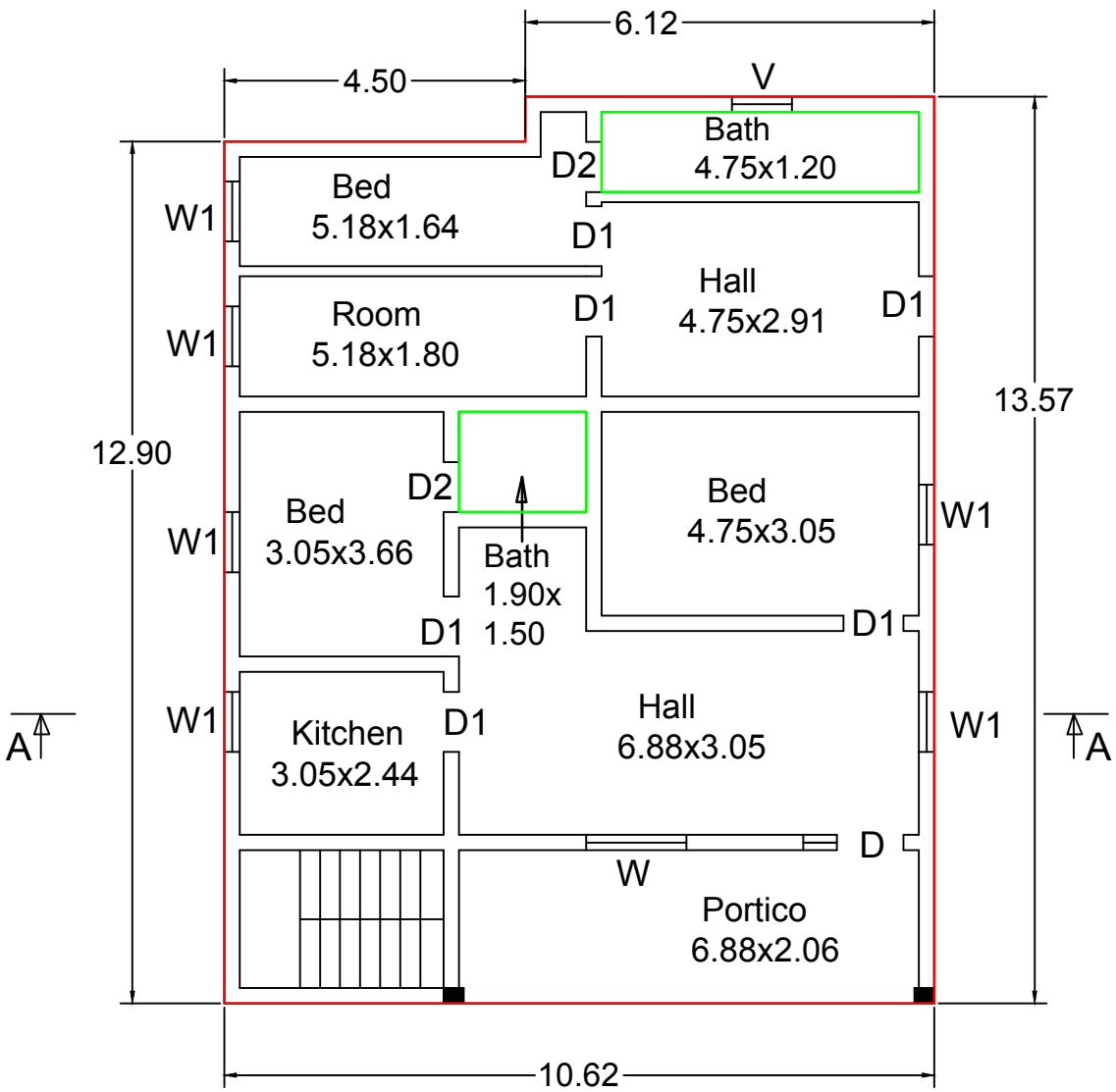
PLAN
