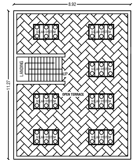
OPEN TERRACE FLOOR PLAN
