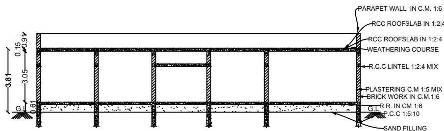
Section On-"AB"
